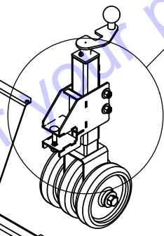
REAR WHEEL ASSEMBLY
