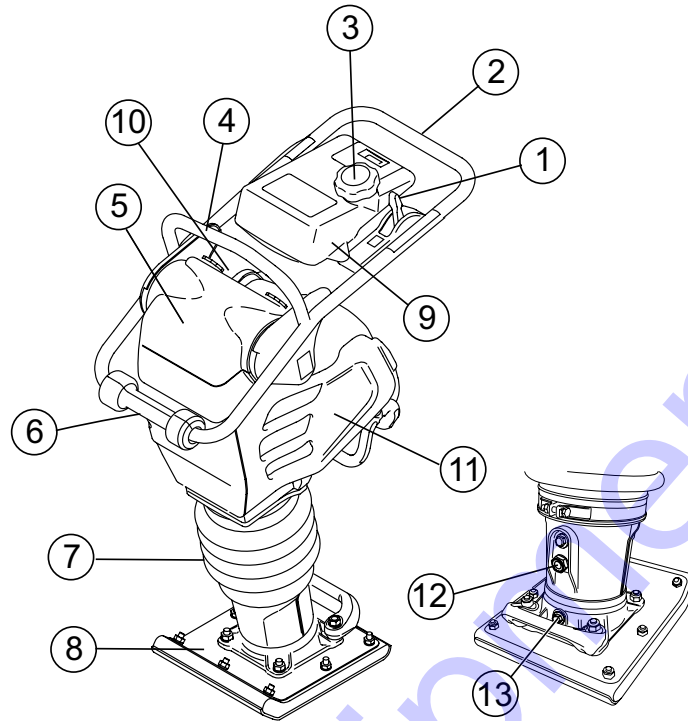
Figure 1. MTX70HDR Rammer
