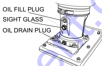
Figure 14. Oil Drain Plug
